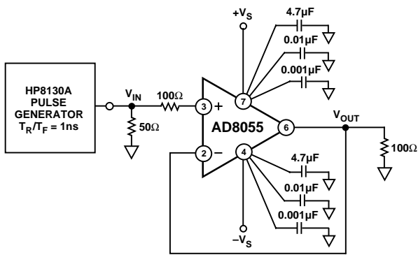
Figure 3. Test Circuit, G = +1 , R_L = 100 \Omega
