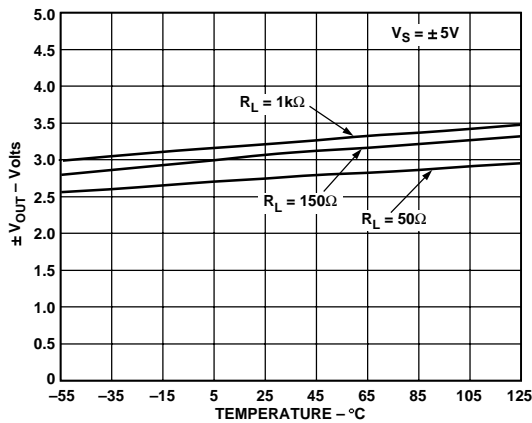
Figure 29. Output Swing vs. Temperature
