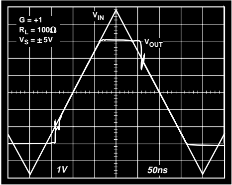
Figure 21. Overload Recovery
