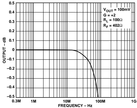
Figure 11. 0.1 dB Flatness
