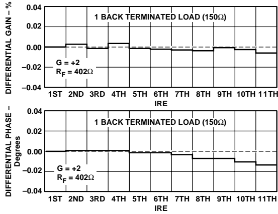
Figure 27. Differential Gain and Differential Phase
