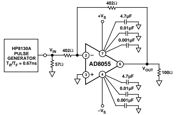
Figure 6. Test Circuit, G = -1 , R_L = 100 \Omega
