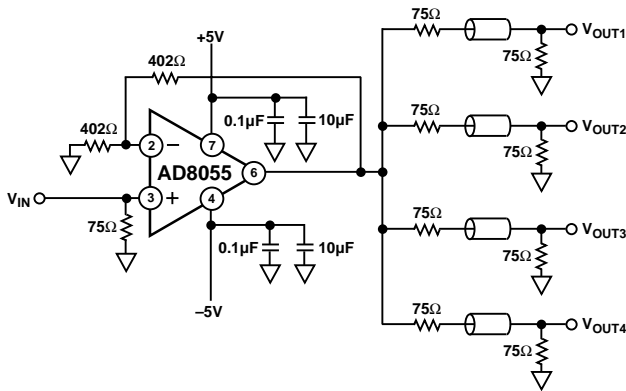
Figure 33. Four-Line Video Driver
